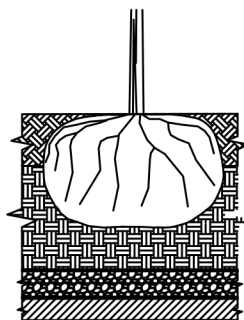
ROOF TOP TREE DETAIL
